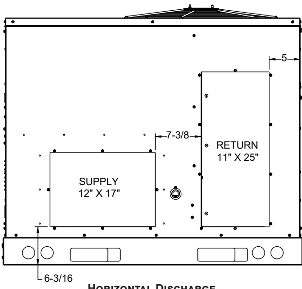
HORIZONTAL DISCHARGE
