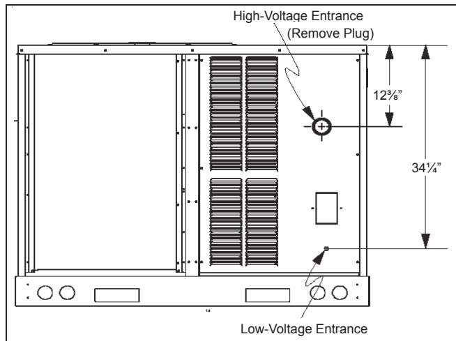
CONDENSER END VIEW
