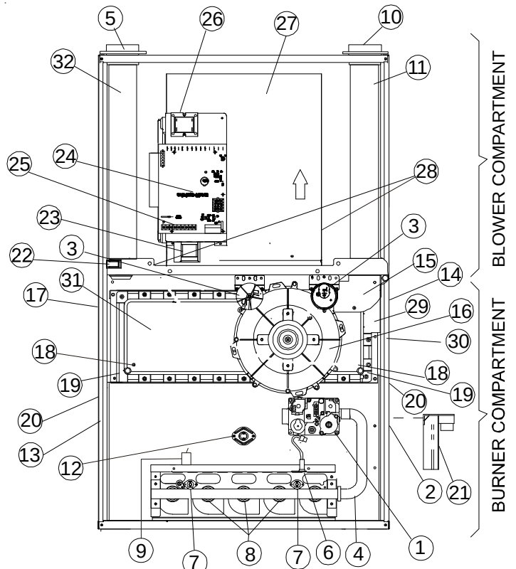
Counterflow /Horizontal
