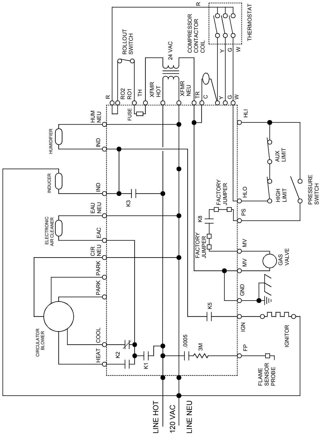
TYPICAL SCHEMATIC GUCA OR GCCA AX MODEL FURNACES WR 50A55-288 INTEGRATED IGNITION CONTROL
