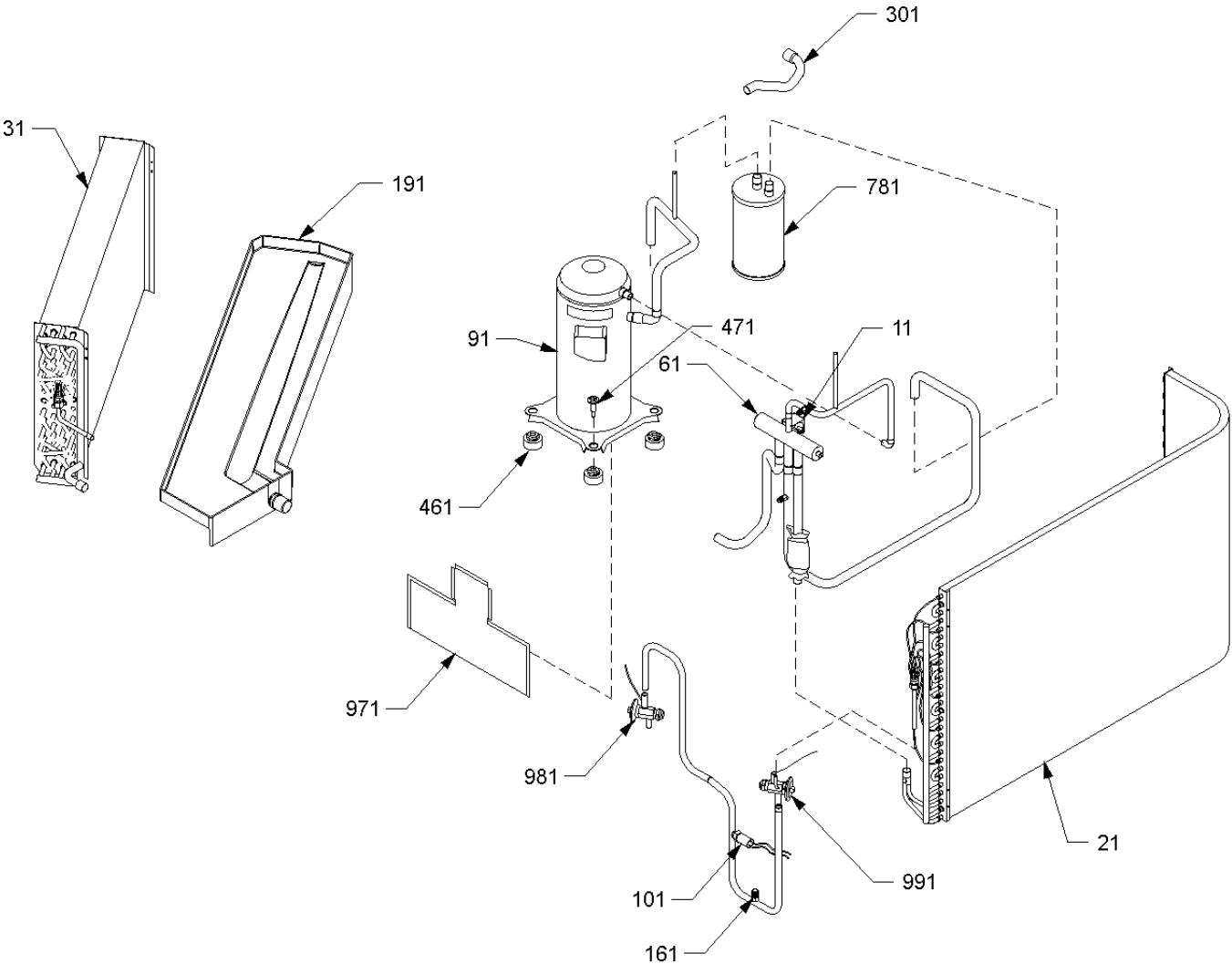
Additional tubing configurations
