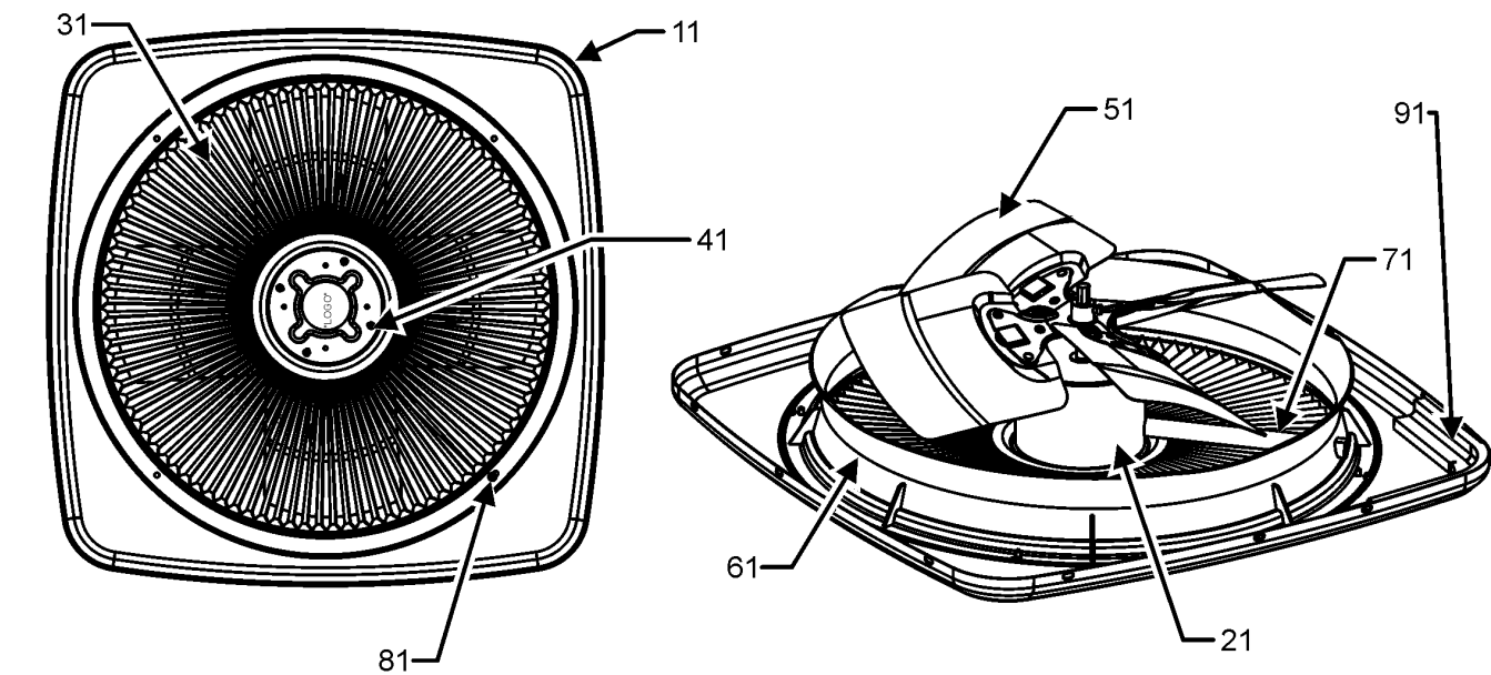
TOP PANEL AND LOUVER PANEL ASSEMBLY
