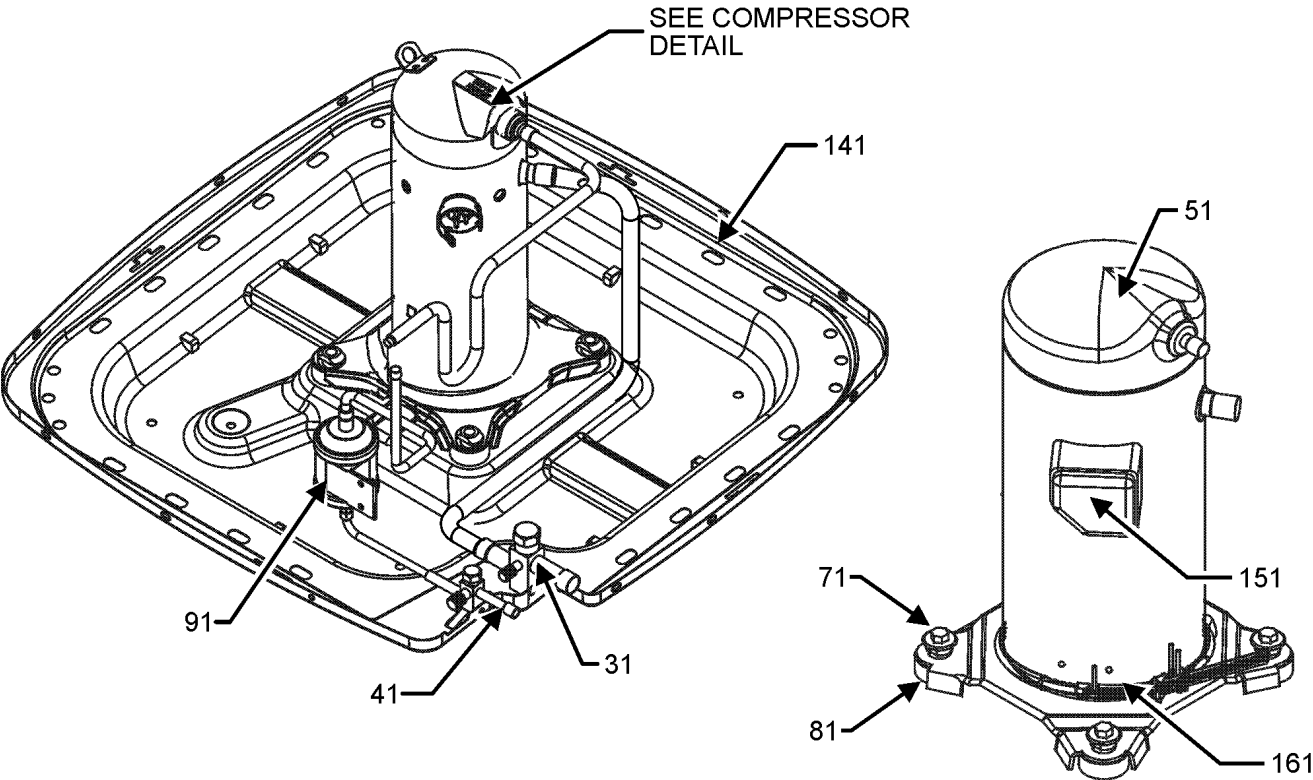
COMPRESSOR DETAIL
