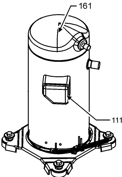
COMPRESSOR DETAIL
