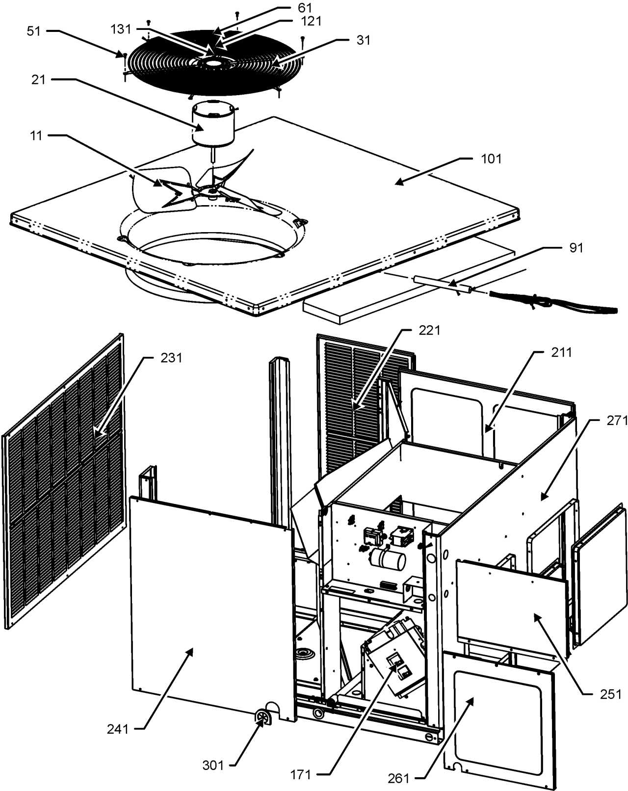
TOP PANEL AND CABINET ASSEMBLY
