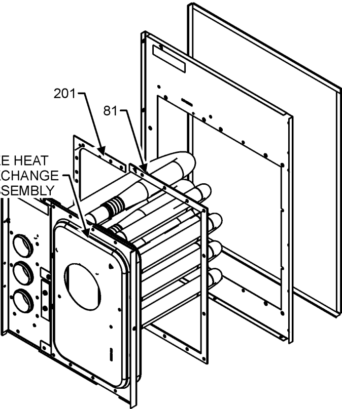
HEAT EXCHANGE ASSEMBLY
