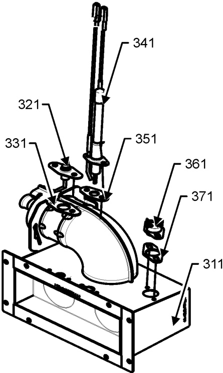
BURNER ASSEMBLY
