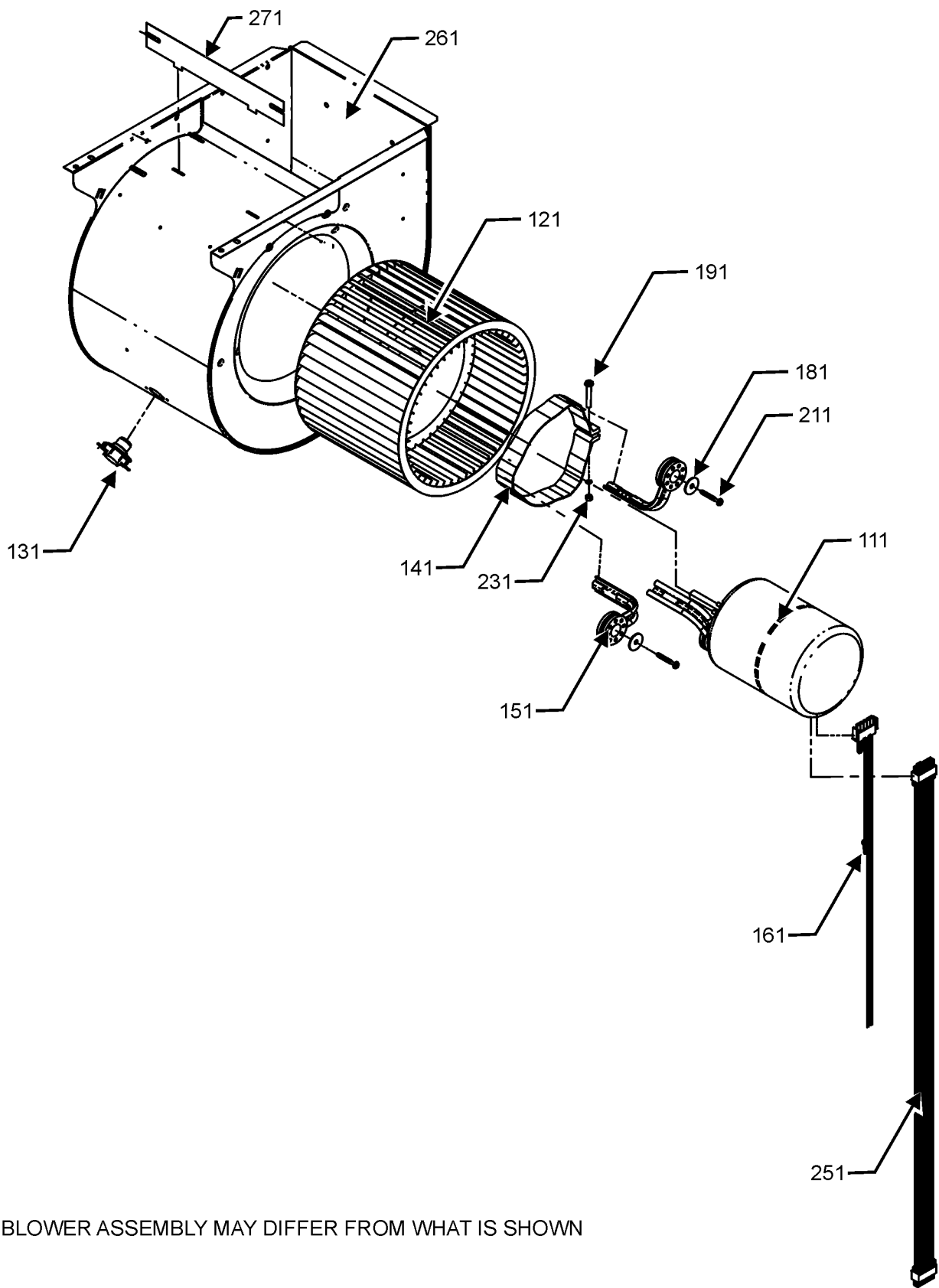
BLOWER ASSEMBLY
