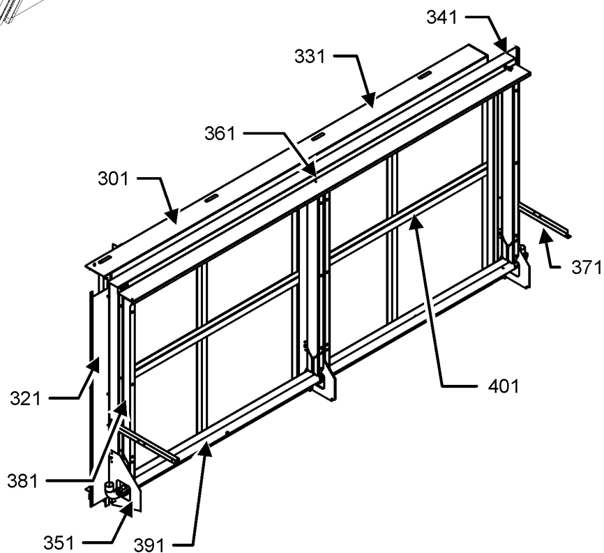
EVAPORATOR ASSEMBLY
