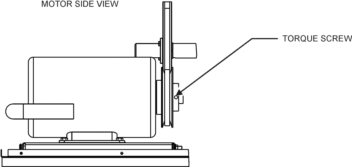
MOTOR SIDE VIEW
