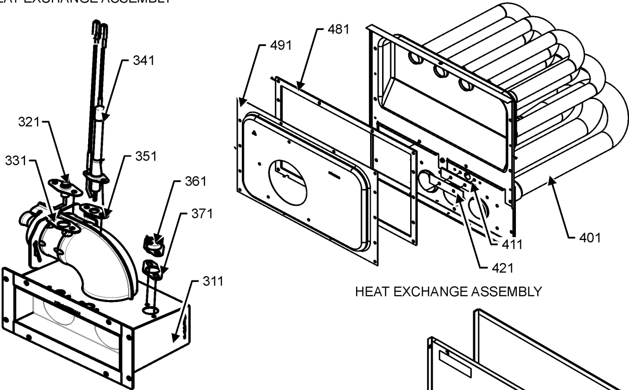
HEAT EXCHANGE ASSEMBLY
