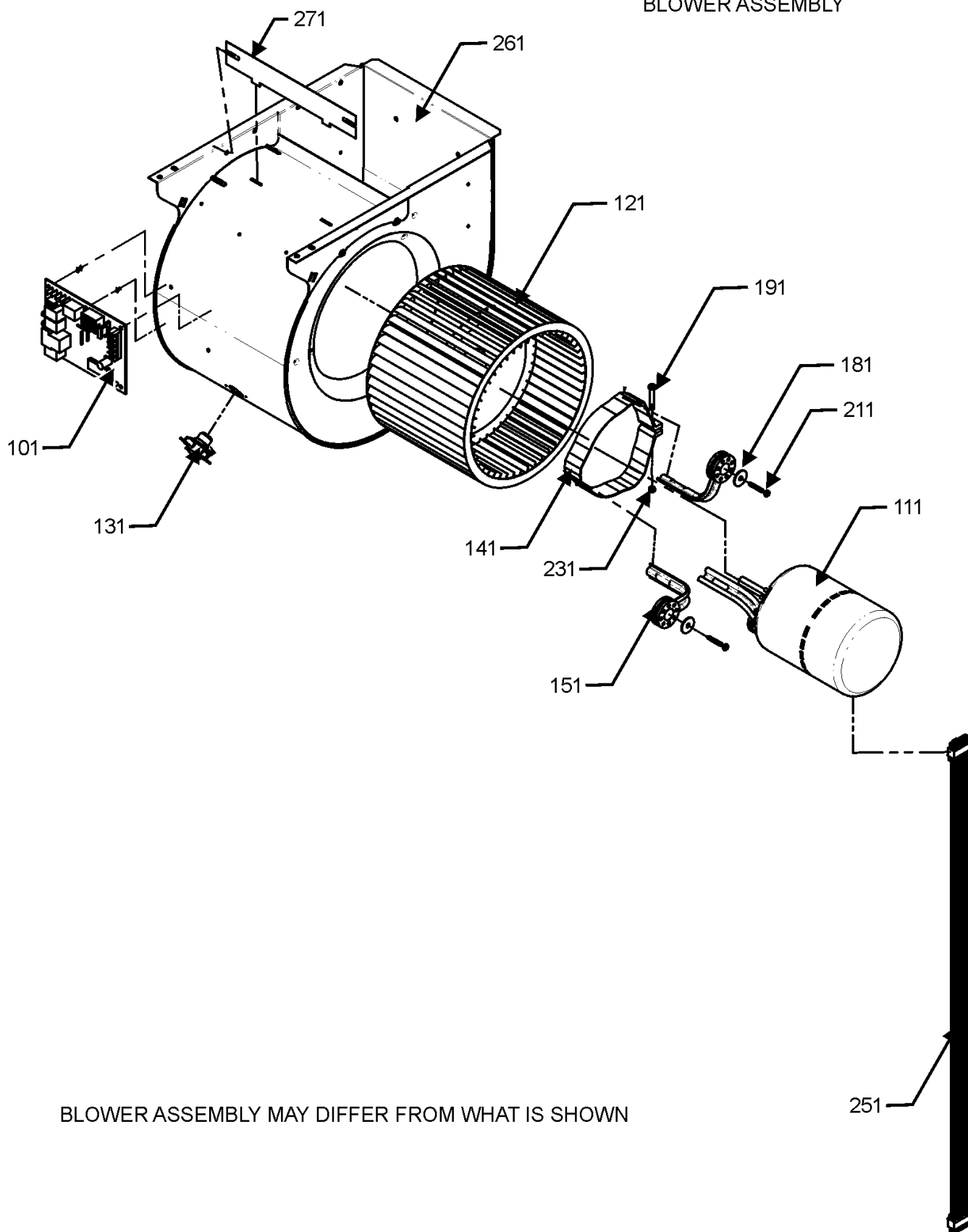
BLOWER ASSEMBLY
